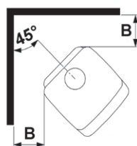
3610 corner installation
